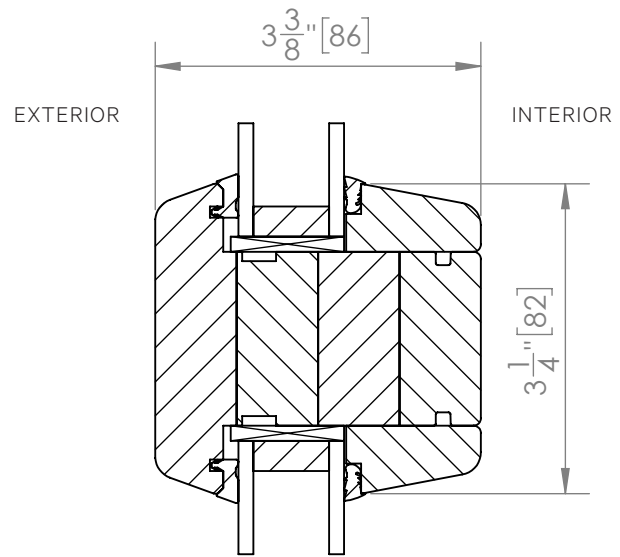
Typical Mullion Profile
